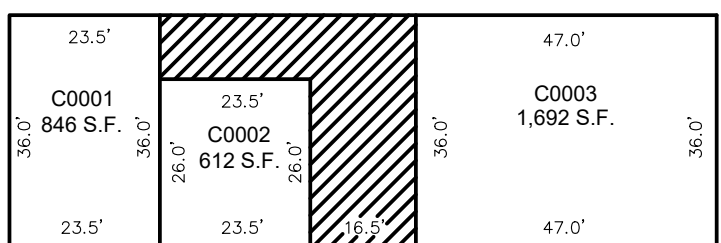
UNIT DETAILS 2424 BRIDGE AVENUE CONDOMINIUM SCALE: 1"=30' BLOCK 315
